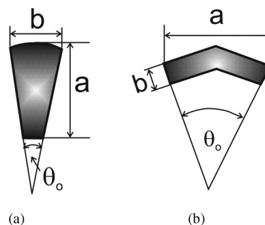
Figure 10. Molecular models used for the calculation of flexoelectric coefficients: (a) pear-shaped molecules; (b) banana-shaped molecules.
